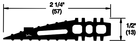
Beveled vinyl nosing for surface mounted installation
