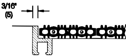
Recessed frame MF-150, MF-151, MF-153, MF-159
