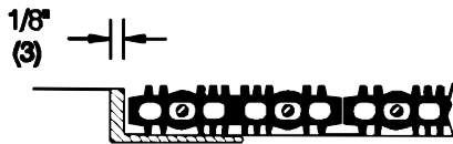
Recessed frame MF-166
