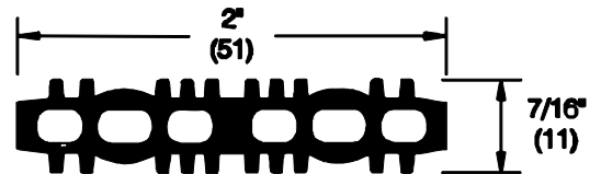
Square vinyl nosing for recessed installation
